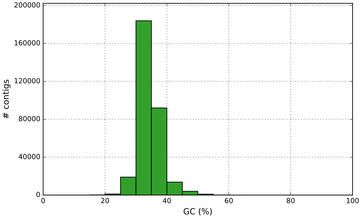
duck4.1 GC content
