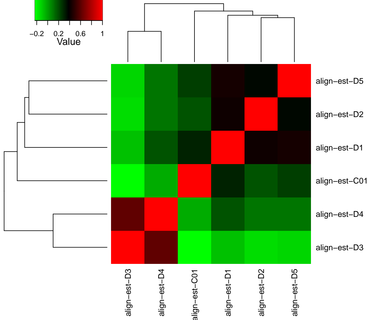
sample correlation matrix diffExpr.P1e-3_C2.matrix.log2
