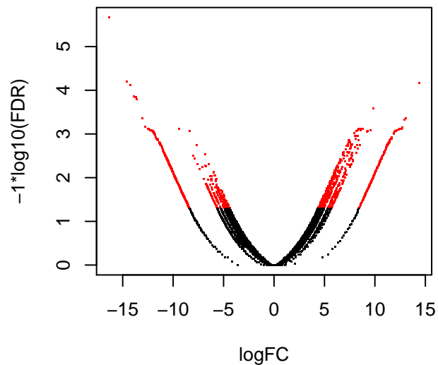
Volcano plot
