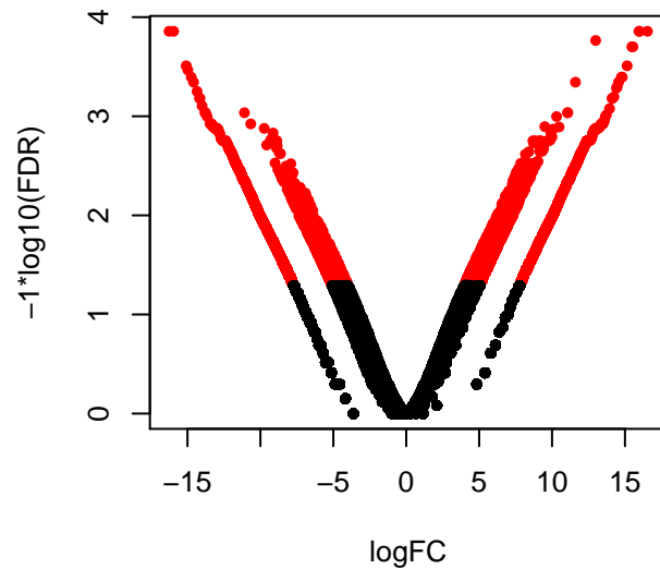
Volcano plot
