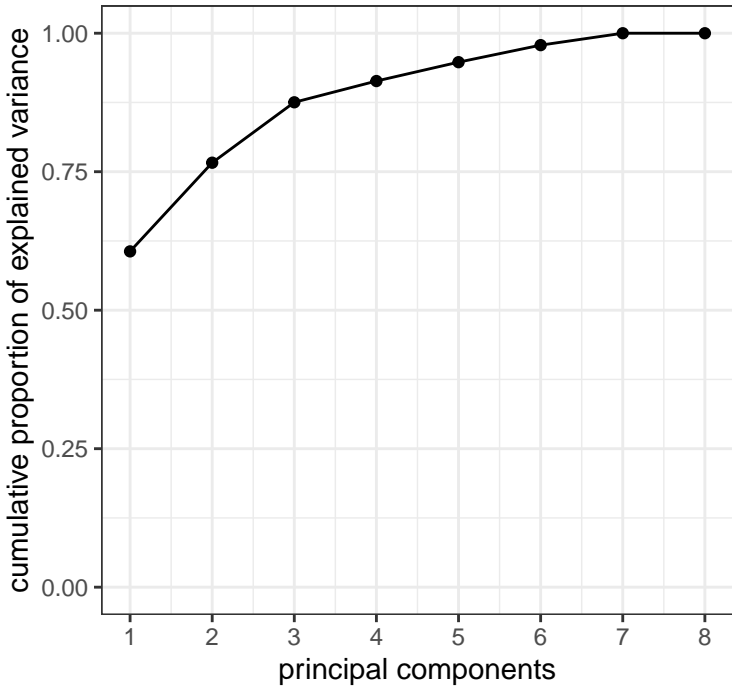
Scree plot for the samples PCA
