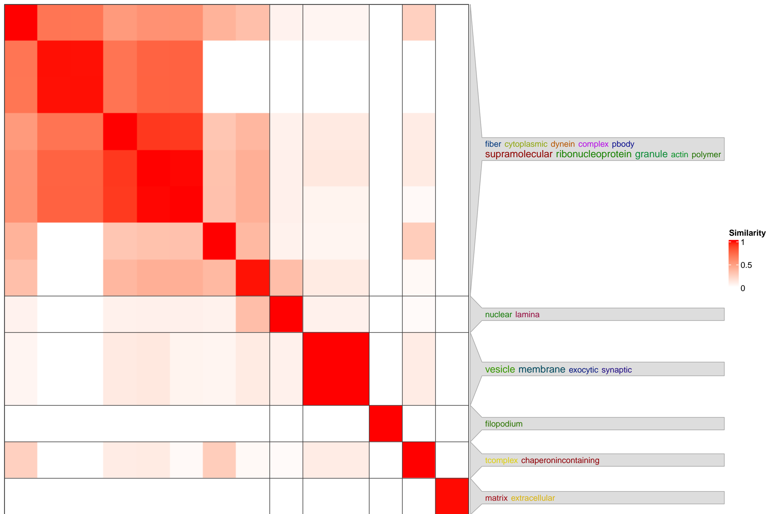
14 GO terms clustered by 'binary_cut'
