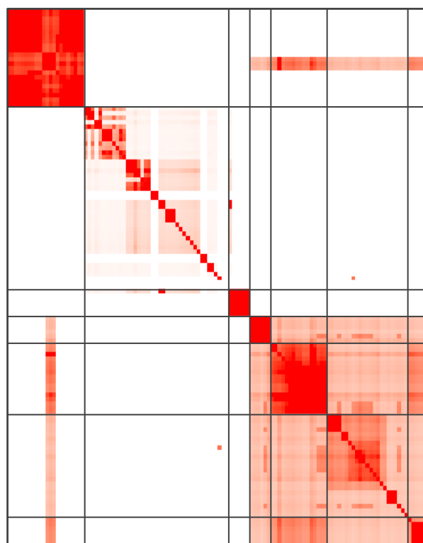
120 terms clustered by 'fast_greedy'
