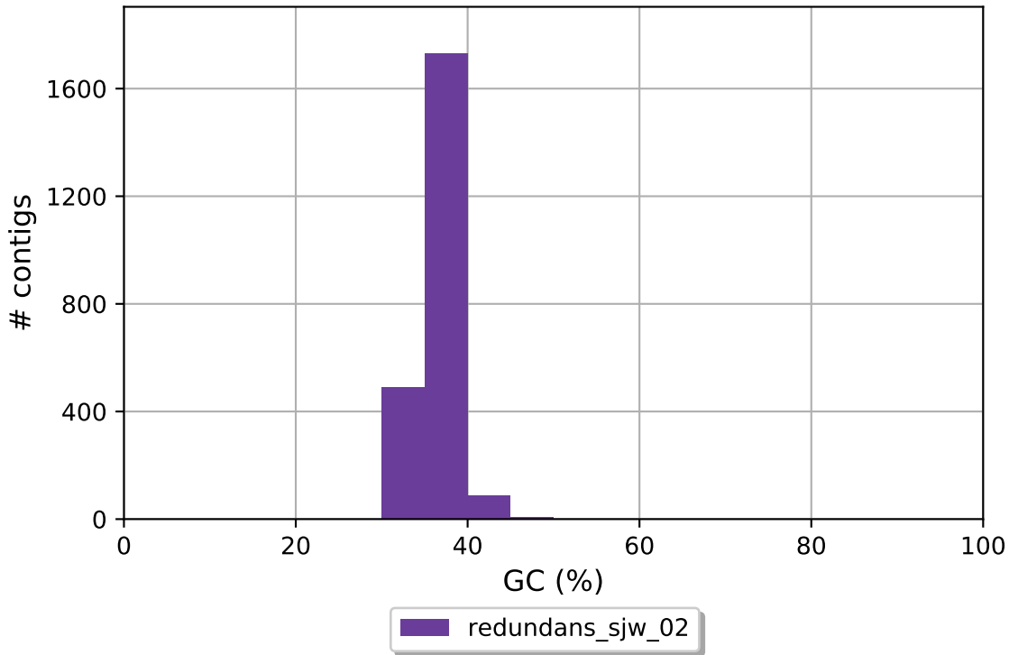
redundans_sjw_02 GC content
