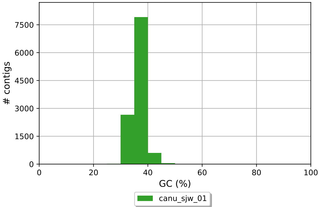
canu_sjw_01 GC content
