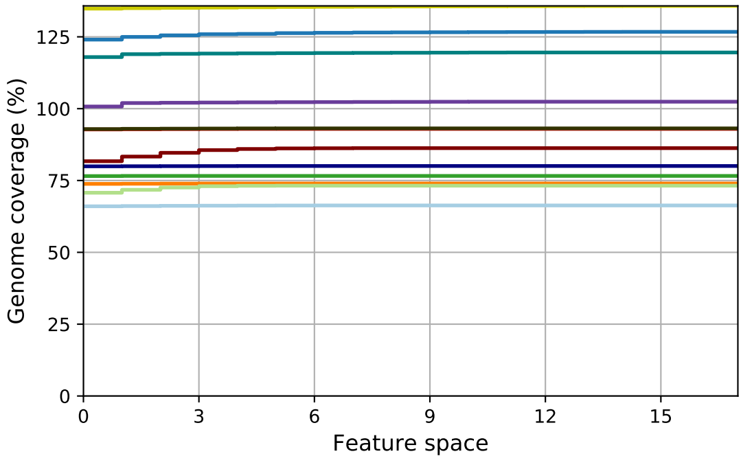
FRCurve (misassemblies)
