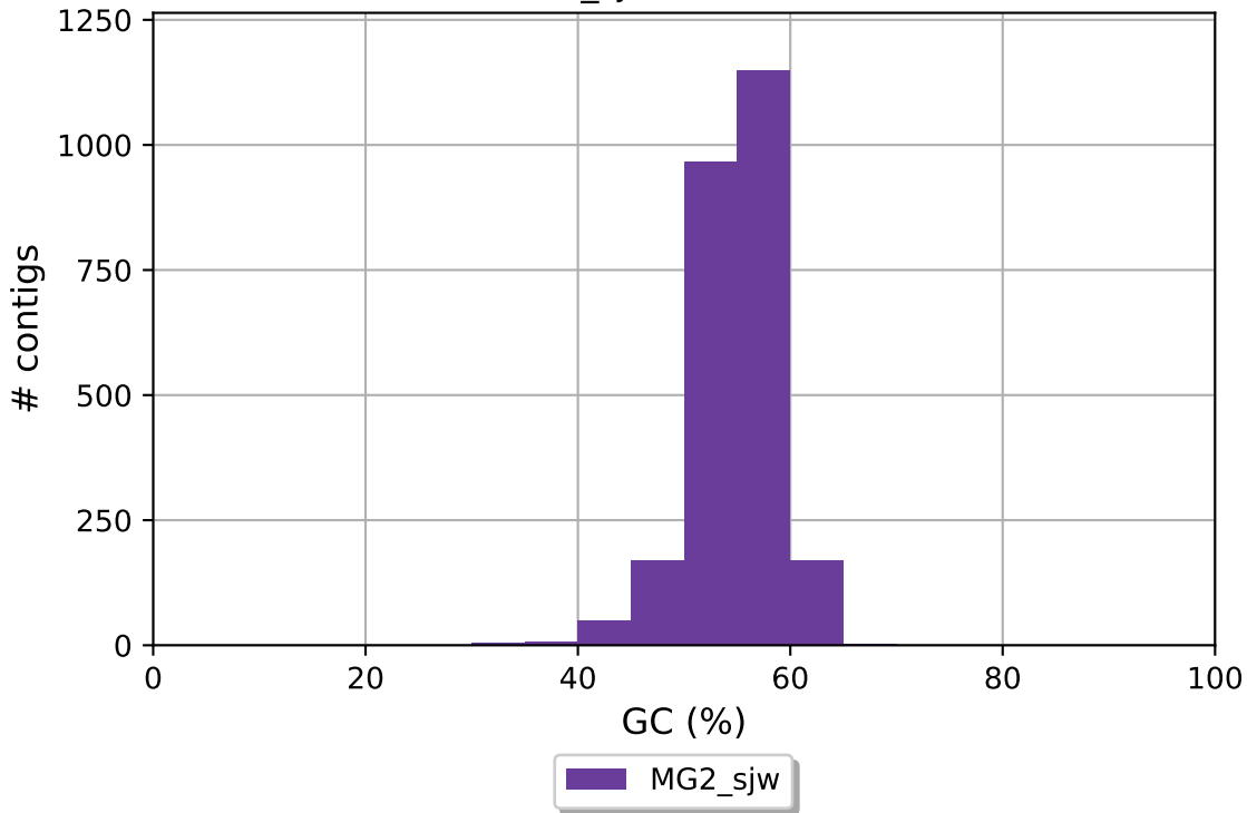
MG2_sjw GC content
