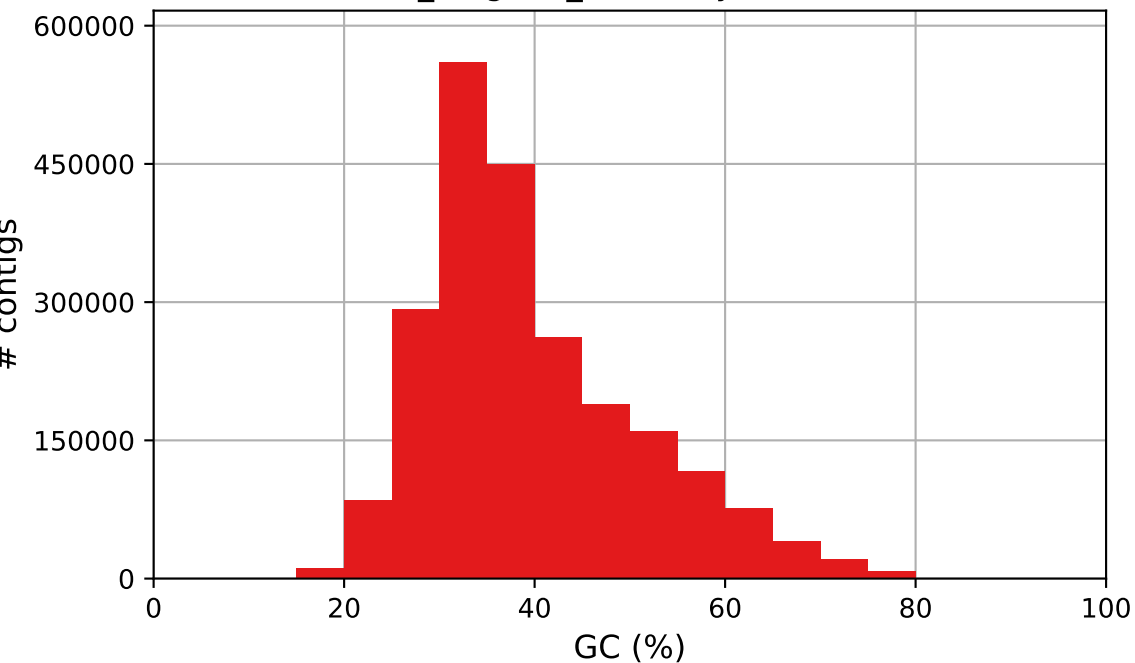
meta_megahit_assembly GC content
